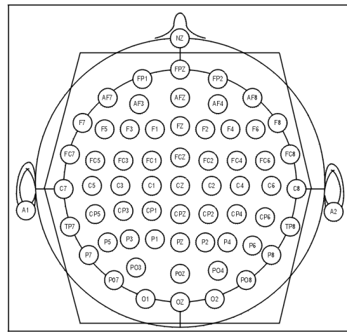
Fig. 4. Electrode positions
