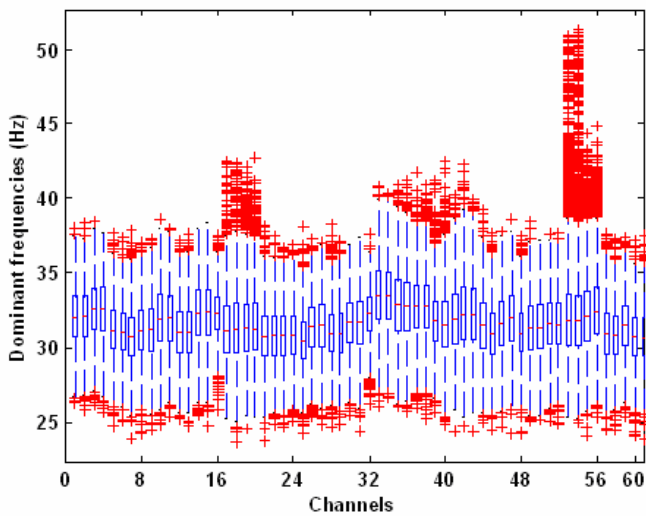
Fig. 6 Box-plot of dominant gamma band frequencies given by the MUSIC algorithm
